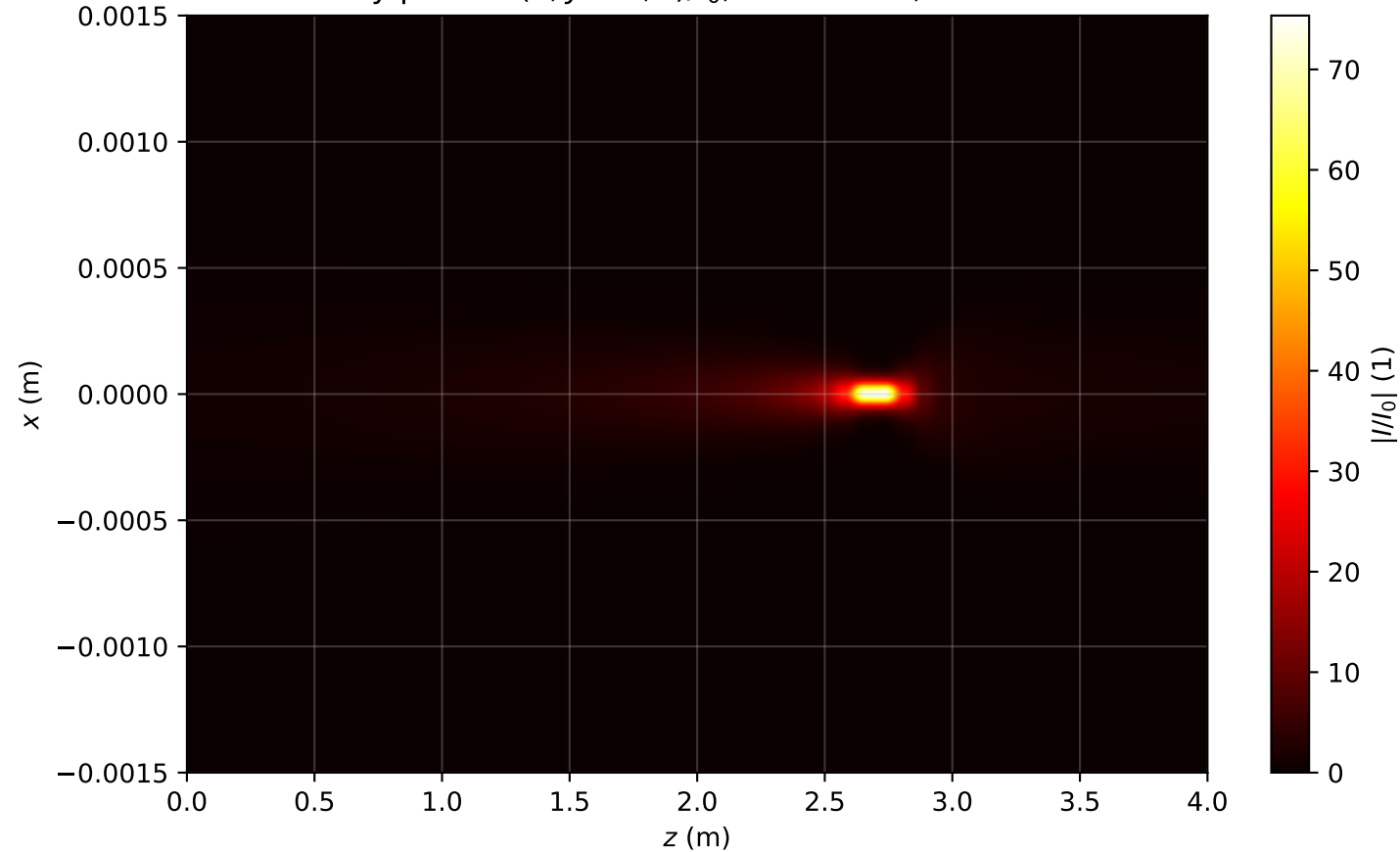
Intensity profile I(x, y = 0, z)/I_0 , P_{in}=1.2P_{cr} , artificial time
